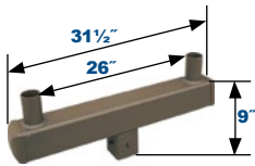
5" Twin Square Vertical Tenon TS5TVT
