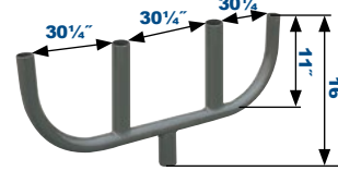
180° Quad Bullhorn TSQ180BH
