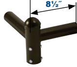
Twin Spoke Bracket, 90° Arms TSB290SZ
