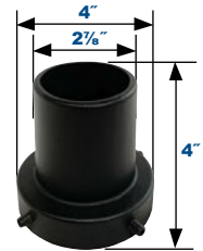
Retrofit Tenon Adaptor for TSRTNB
