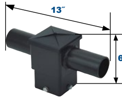
5" 180° Twin Square Horizontal Tenon TS5T180HT
