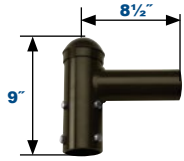
Single Spoke Bracket TSB1SZ
