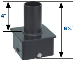
5" Single Square Vertical Tenon - 2 1/2" Dia. TS5SVTZ
