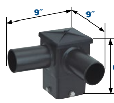
5" 90° Twin Square Horizontal Tenon TS5T90HT
