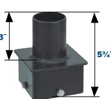
5" Single Square Vertical Tenon - 2 1/2" Dia. TS5S3SVTZ
